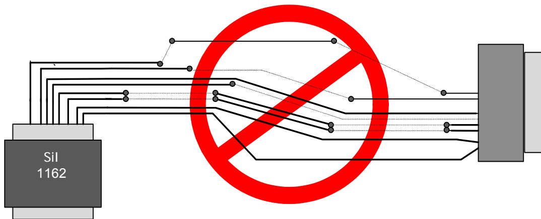
Figure 24. Example of Incorrect Differential Signal Routing
