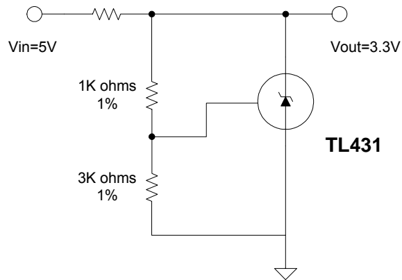
Figure 17. Voltage Regulation using TL431
